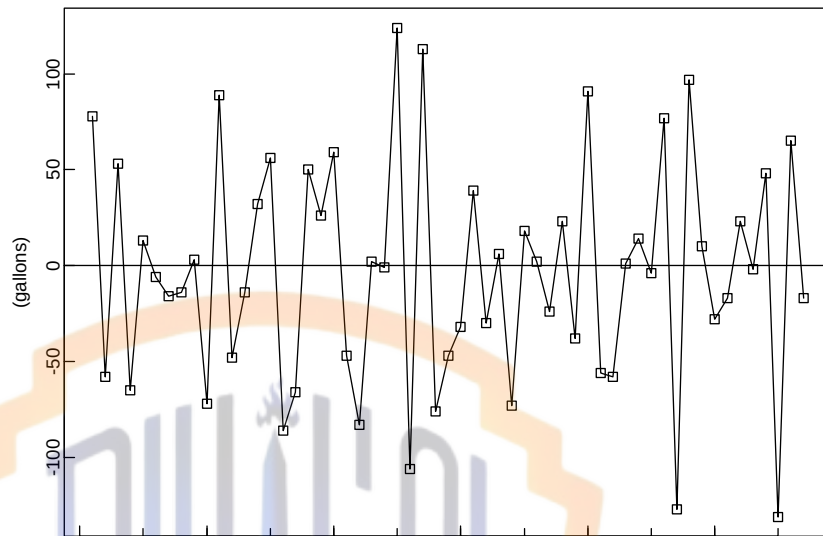
Figure 3-5 Time series of the overshoots in Example 3.2.8.
